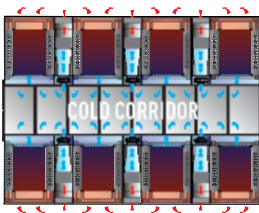
Open loop
